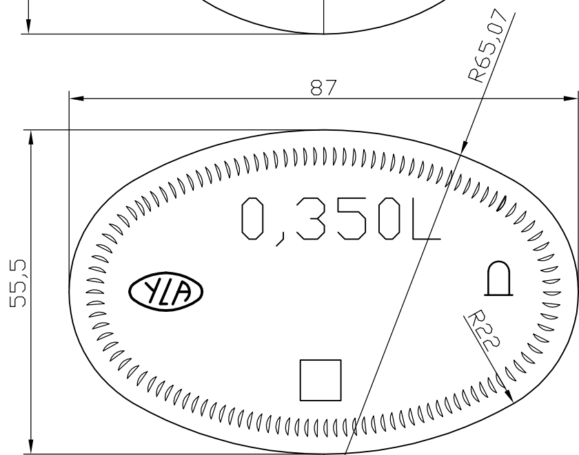
SECTION C-C and BOTTOM VIEW
